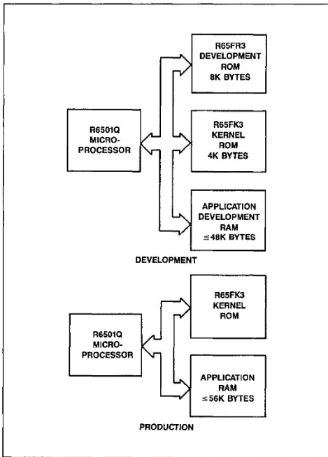
Figure 4. R65FR3 and R65FK3 Configuration 3 Block Diagrams
