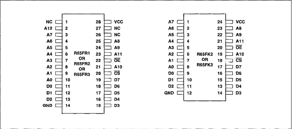
RSC-FORTH ROM Pin Assignments
