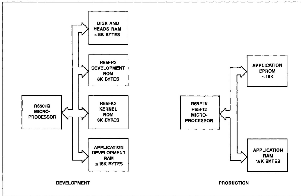
Figure 2. R65FR2 and R65FK2 Configuration 2 Block Diagrams
